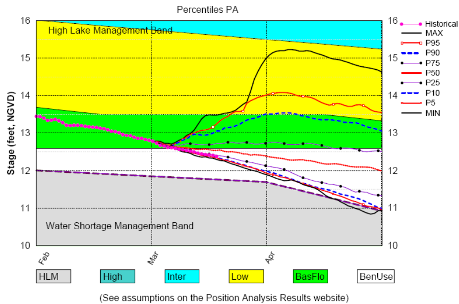
Figure 1. This graph predicts future lake levels based on historical rainfall patterns in South Florida (from the LORS page, https://my.sfwmd.gov/pls/portal/docs/PAGE/PG_GRP_SFWMD_HESM/PORTLET_TECHSUMFILES/lors03162009/img_rpt/projection.pdf ).
